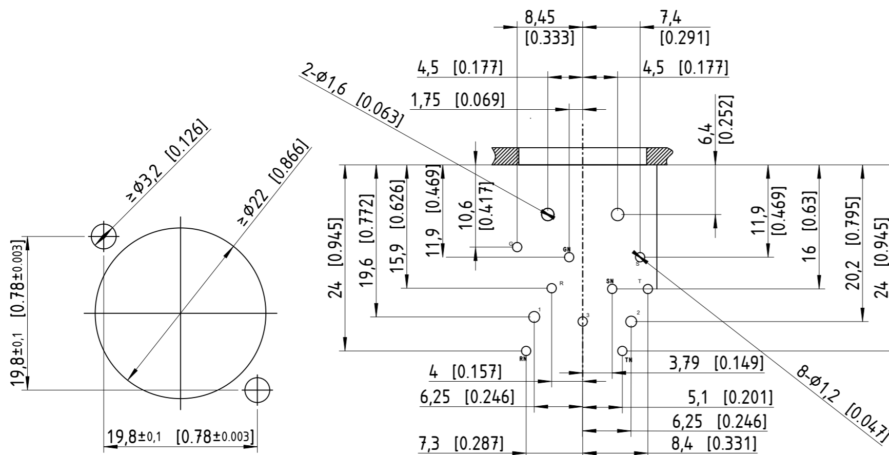
PCB Layout(Component side) tolerance ±0.05 [0.002]
