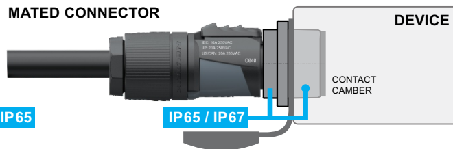
MATED CONNECTOR
